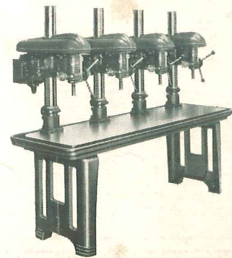
No. 1555 Four Spindle 17" Drill Press and Standard Production Table.
